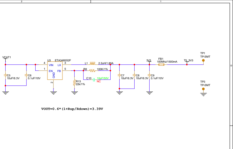
VCAT1转3V3
